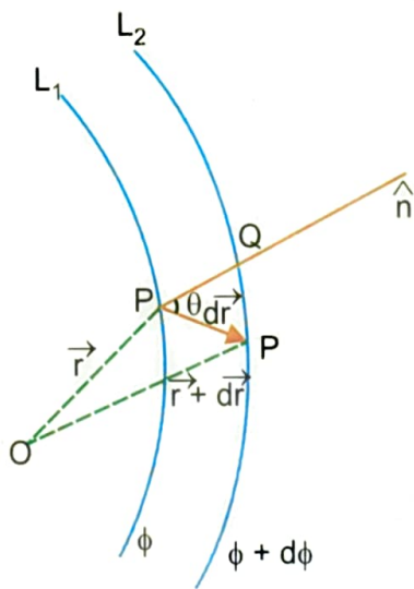
Two-level surfaces L_1 and L_2 through two close points P and P'
