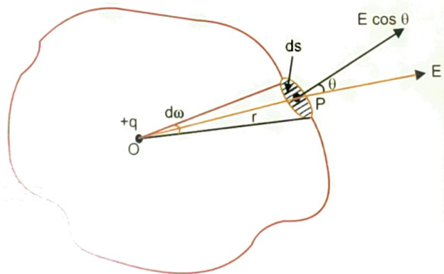
Gauss's theorem
