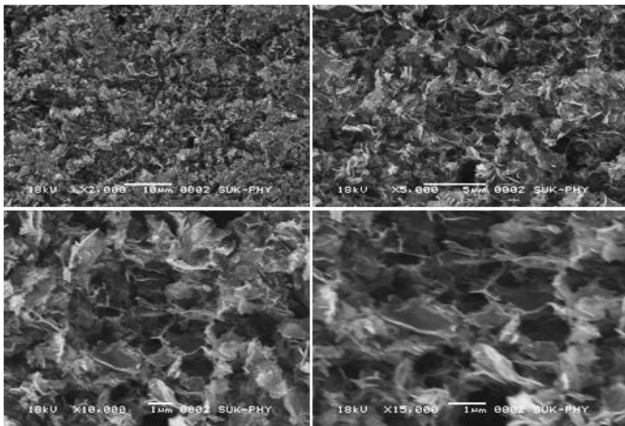
Fig. 4. SEM of coral-rock-like morphology of CZTS.
